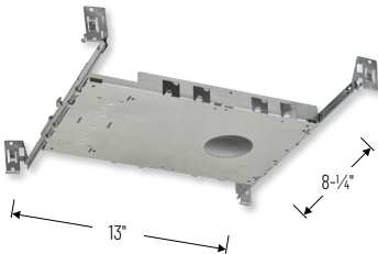
NHIOFK-1 New Construction Frame-In for 1" Remodel Housing
