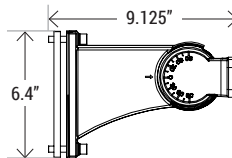
SAM-AL2 Straight Arm Mount for Square Pole
